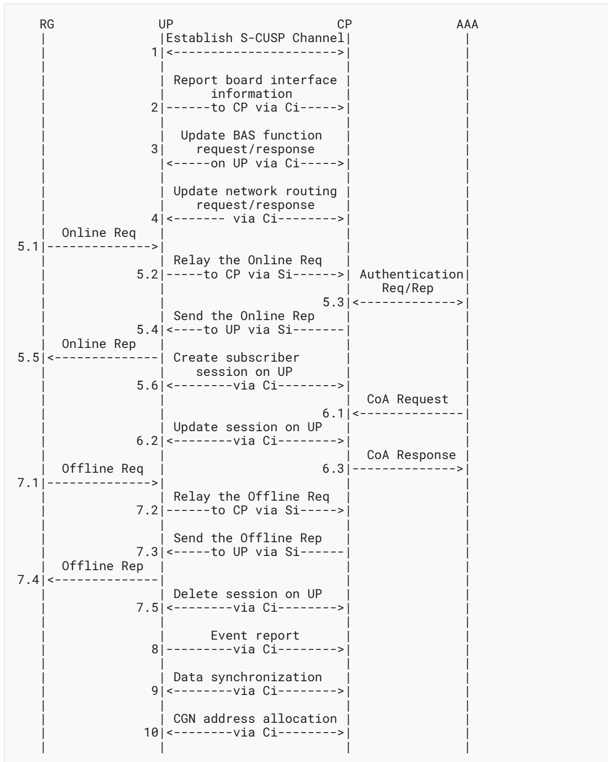
Figure 3: BNG CUPS Procedures Overview
