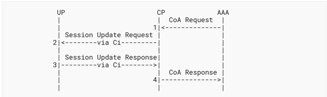
Figure 11: Subscriber Session Update
