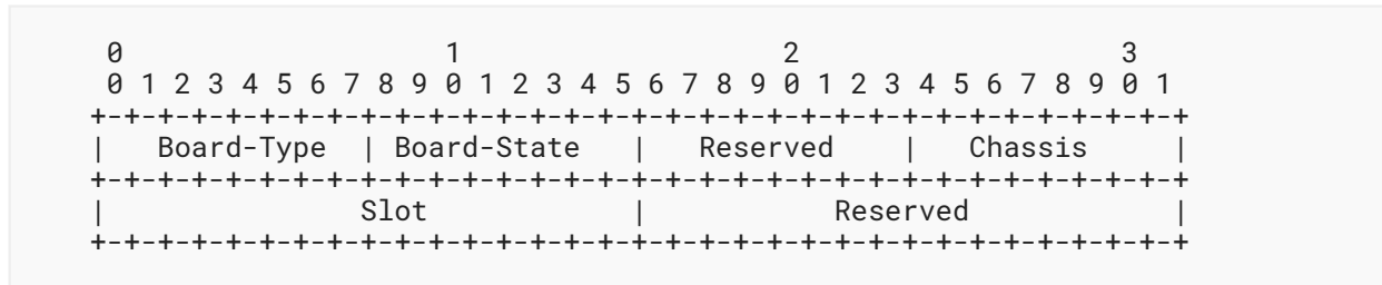
Figure 60: Interface Resource TLV
