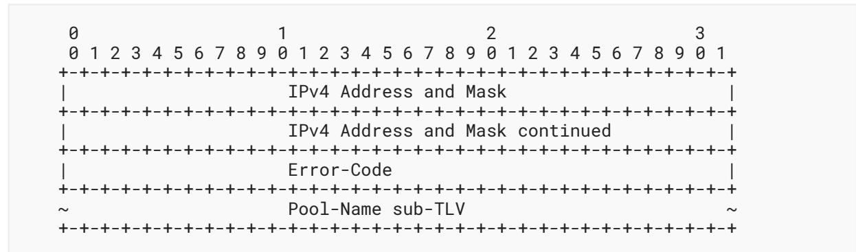
Figure 66: Address Renewal Response TLV
