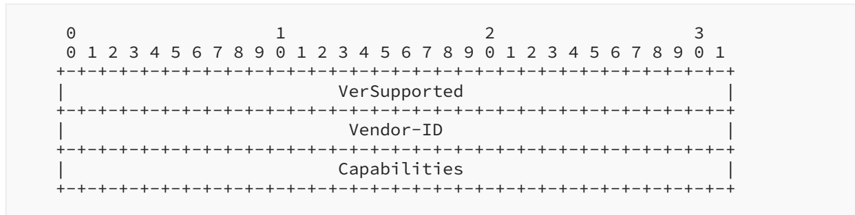
Figure 39: Hello TLV
