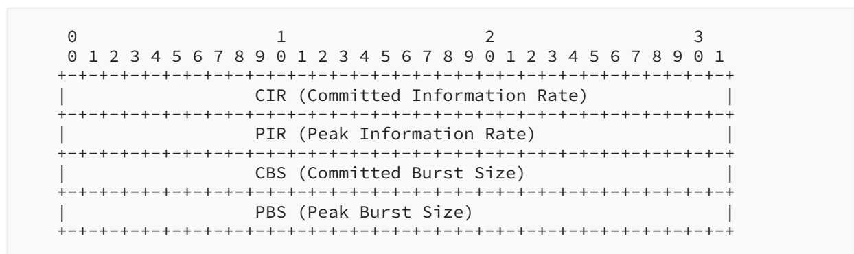
Figure 34: Ingress-CAR Sub-TLV
