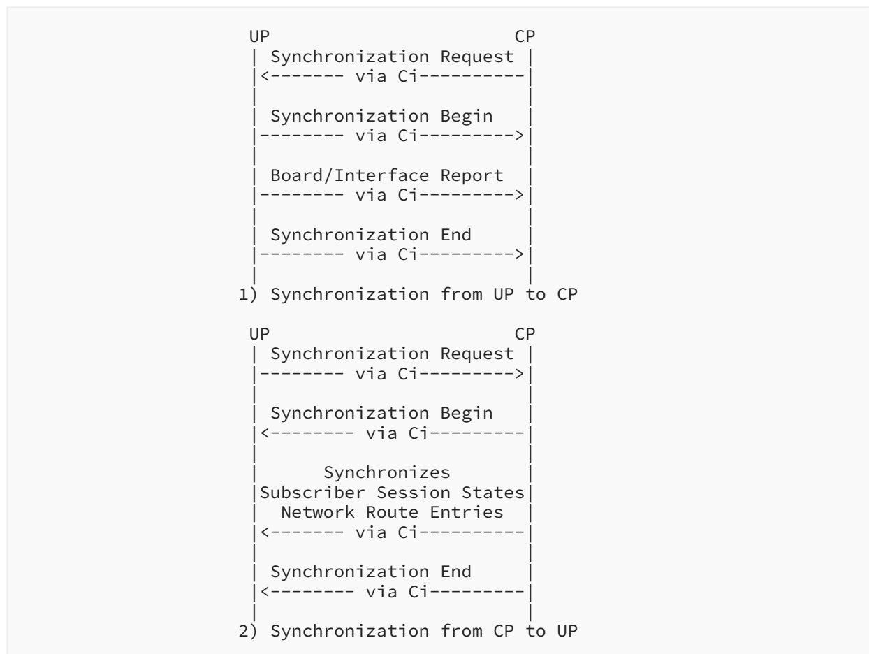
Figure 9: Data Synchronization
