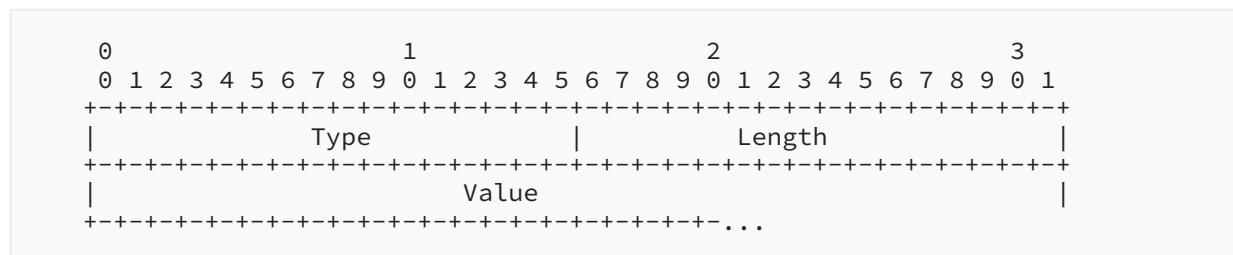
Figure 33: Sub-TLV Header
