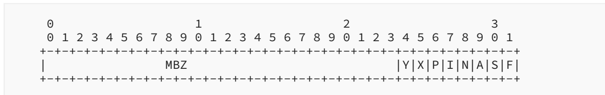
Figure 43: Interface Flags
