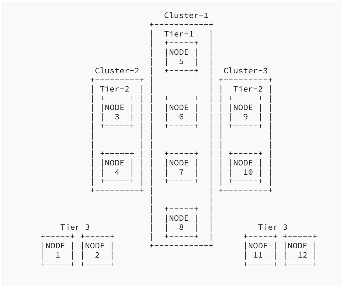
Figure 3: iBGP Sessions with Reflection and Next-Hop-Self
