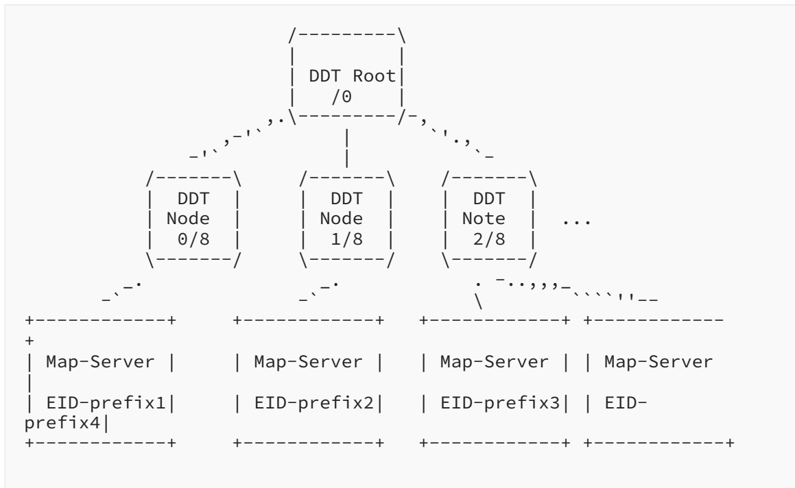
Figure 3: A Schematic Representation of the DDT Tree Structure
