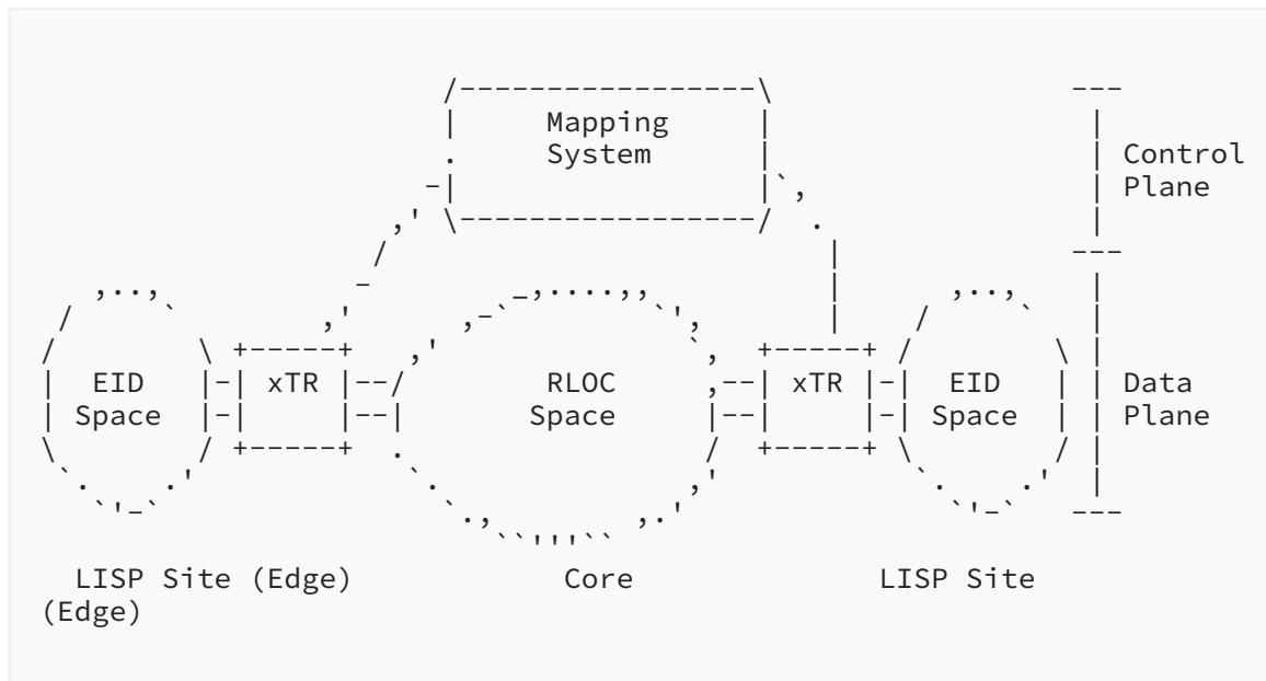
Figure 1: A Schema of the LISP Architecture
