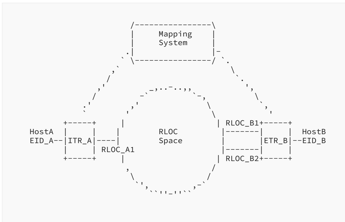
Figure 2: Packet Flow Sequence in LISP
